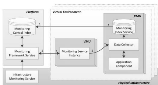
Figure 13: IRMOS Adaptable monitoring framework
